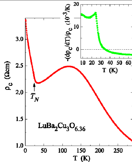
Fig. 1 Out-of-plane resistivity, \rho_c(T) , of a \text{LuBa}_2\text{Cu}_3\text{O}_{6.36} single crystal. The sharp growth of the resistivity upon cooling below \approx 25 K is caused by the AF ordering. Inset : anomaly in the normalized derivative (d\rho_c/dT)/\rho_c associated with the Néel transition
