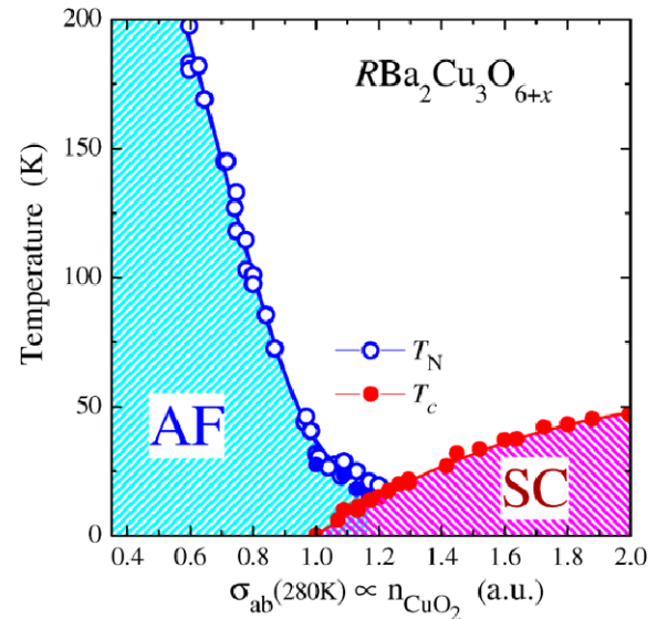
Fig. 2 Phase diagram of \text{RBa}_2\text{Cu}_3\text{O}_{6+x} ( R = \text{Lu, Tm, Y} ) crystals near the AF–SC transformation. The AF and SC transition temperatures, T_N and T_c , are presented as a function of the in-plane conductivity \sigma_{ab}(280\text{ K}) which is a good measure of the hole density in the shown doping region [20]. The Néel temperature was determined either at the position of the jump (middle point) in the derivative d\rho_c/dT (open circles), or at the position of the negative peak in d\rho_c/dT (solid circles)
