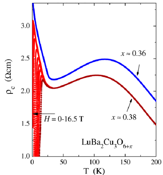
Fig. 3 Out-of-plane resistivity of one and the same \text{LuBa}_2\text{Cu}_3\text{O}_{6+x} single crystal for two oxygen concentrations near the AF–SC transformation. For the superconducting composition x = 0.38 , the data were taken at several magnetic fields—from zero up to 16.5\text{ T} —applied along the c axis. The sharp upturn in the resistivity associated with the Néel transition shows up as the superconductivity is suppressed with the magnetic field
